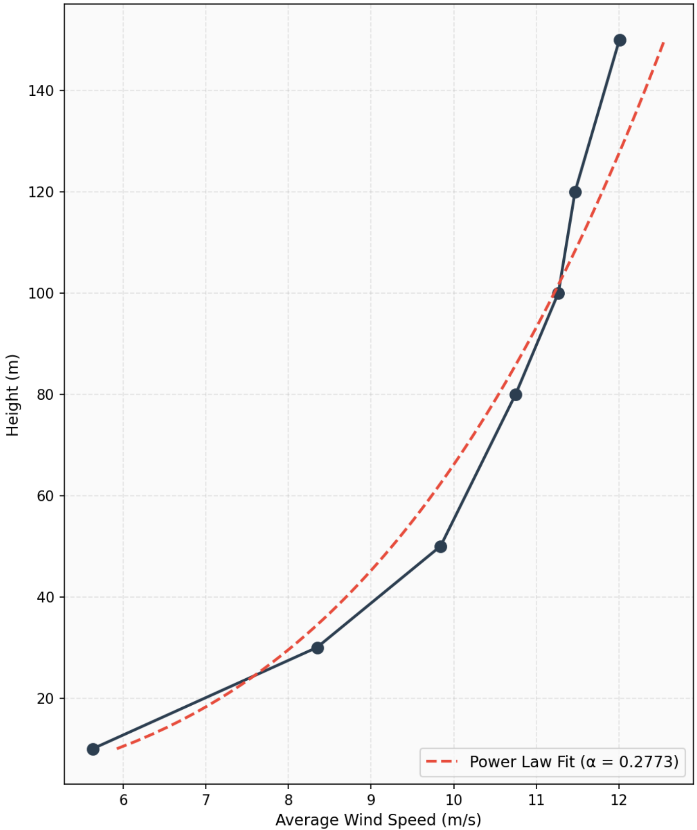
Sonapur — Wind Shear Profile
