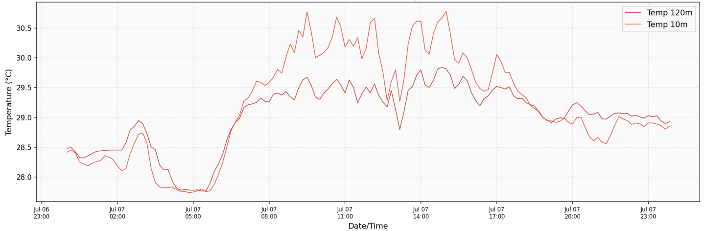
Sonapur — Time Series: Temperature
